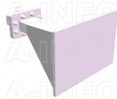
LB-187-15-C-TFSP0 Standard Gain Horn Antenna 3.95-5.85GHz 15dB Gain TNC Female
